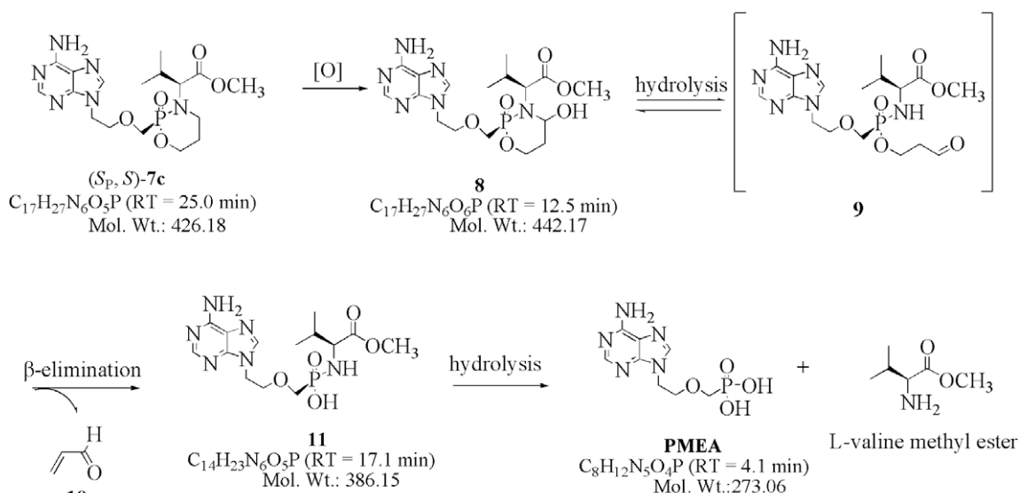
Figure 2. Possible metabolic pathway of ( S P , S )- 7c .
