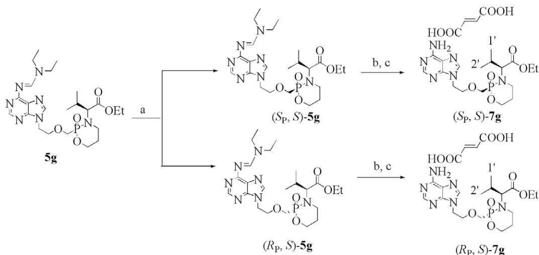
Scheme 2. Reagents: (a) chromatographic resolution; (b) \text{AcOH} , reflux, 2 h; (c) fumaric acid, \text{MeCN} , reflux, 1 h.
