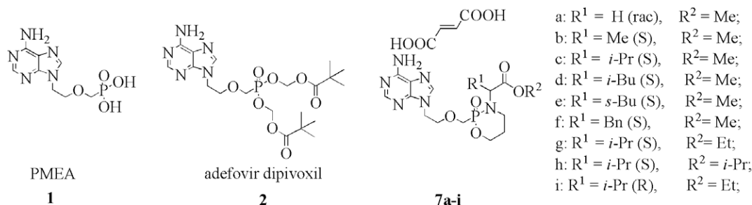
Figure 1. Structures of PME A ( 1 ), adefovir dipivoxil ( 2 ) and compounds 7a-i .
